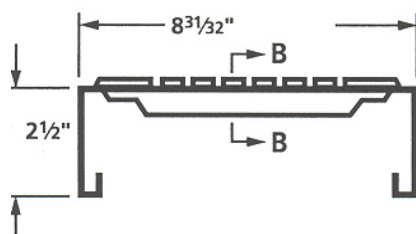
Standard Section Double-Male Leg
